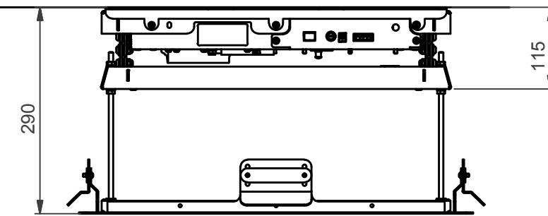
UP POSITION
