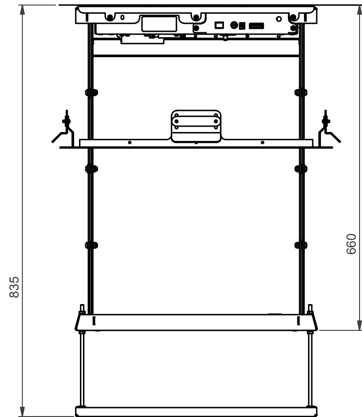
DOWN POSITION
