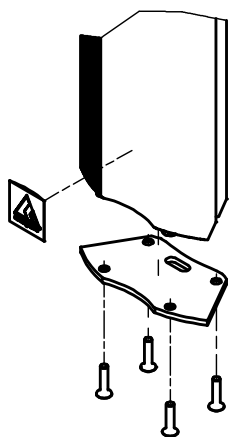
Detail "C"
